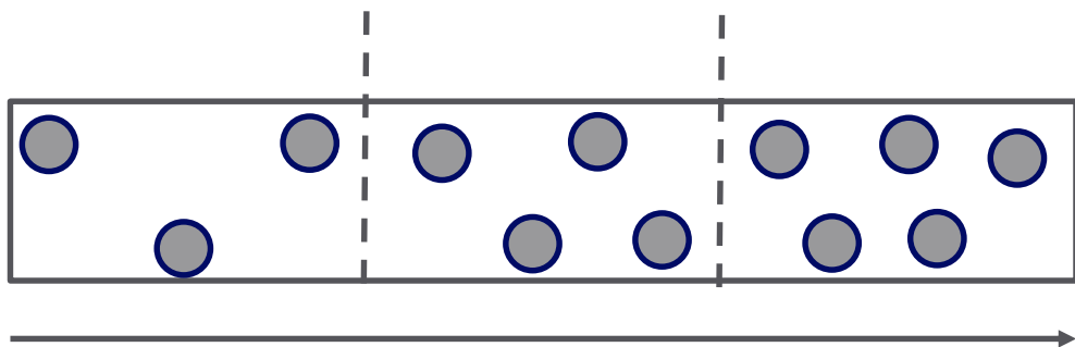
Same pressure but increasing compressibility
