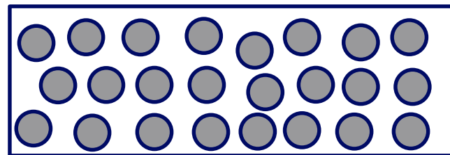
More molecules in the same space
